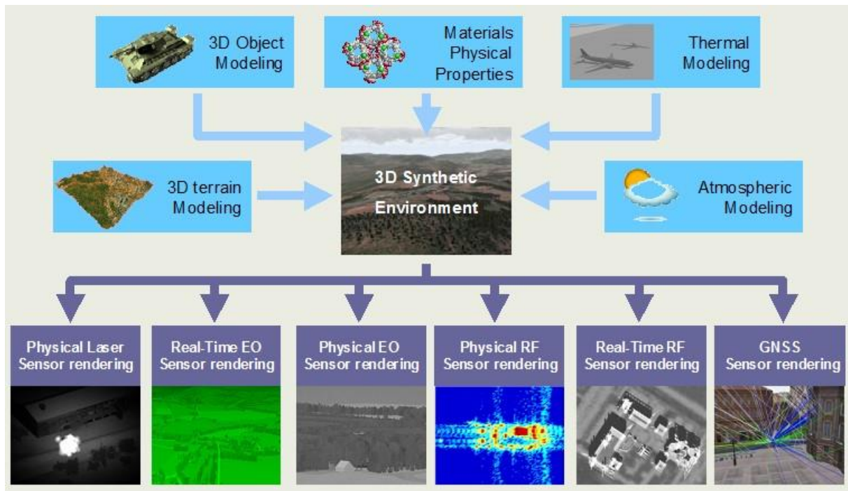
Figure 6. Global architecture of OKTAL-SE SE-Workbench.
