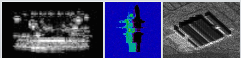
Target (vehicles, buildings) SAR signature using OKTAL-SE tools
