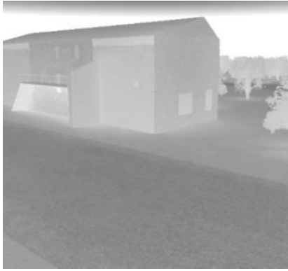
Figure 11: High quality SE-RAY-IR spectral images using photon maps enhancement
